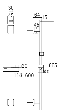
AMBA-801 SUS 304 Shower Rail Only (ABS Holder) Square • Stainless Steel SUS 304 • Hairline • 1 pc/box, 12 pcs/ctn RM197.00
