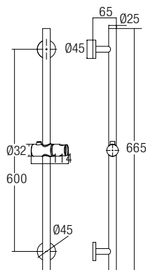
AMBA-800 SUS 304 Shower Rail Only (ABS Holder) Round • Stainless Steel SUS 304 • Hairline • 1 pc/box, 12 pcs/ctn RM143.00
