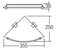
AMBA-301 Corner Glass Shelf • Brass • Chrome • 1 pc/box, 10 pcs/ctn RM131.00
