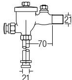
AMFV-500 Exposed Urinal Flush Valve c/w Rubber Spud & Straight Proliferated Pipe • Brass • Chrome • 1 pc/box, 24 pcs/ctn RM230.00
